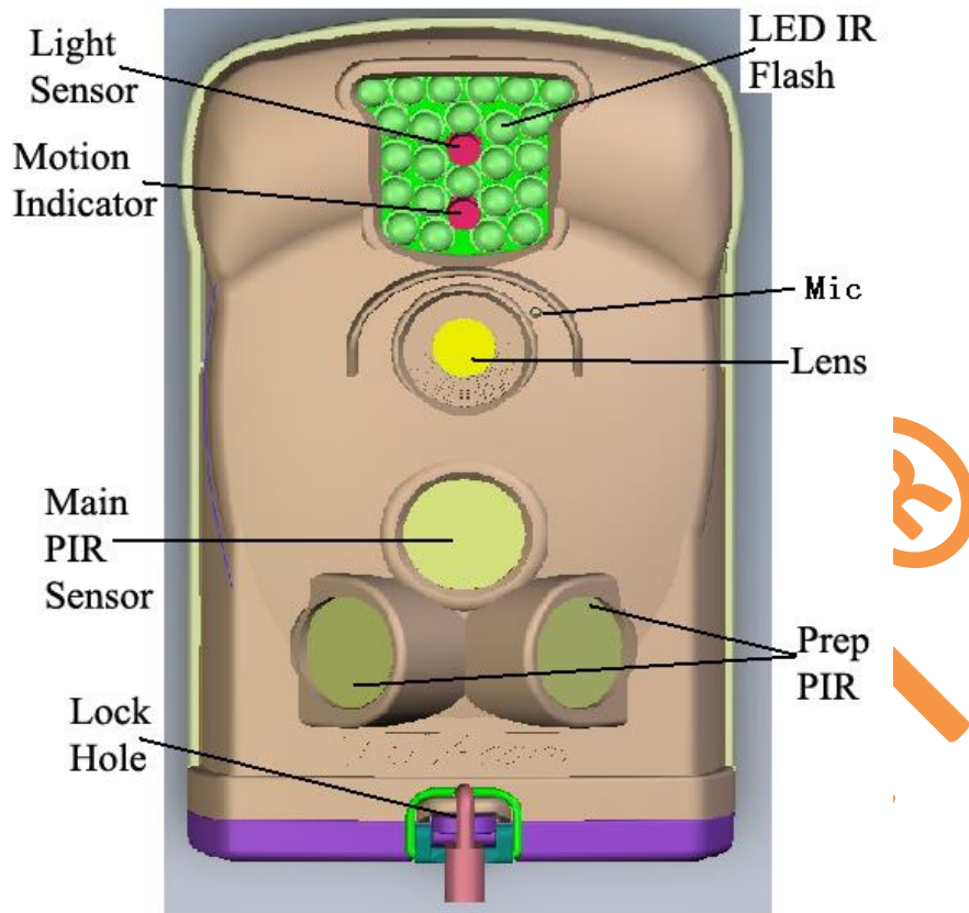
Figure 1.1: Front View of Ltl-6210M
